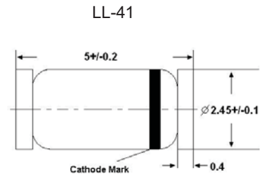
LL-41 Glass case MELF Dimensions in mm
